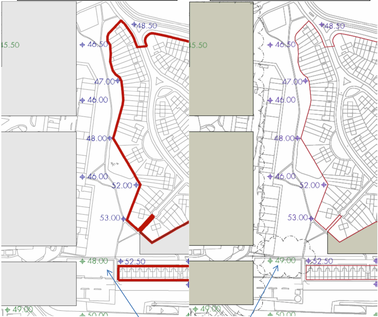
Detail from Existing Levels Parameter Plan 006
